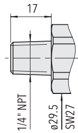
8292.XX.XX30.XX.XX.XX (≤ 1000 bar)
